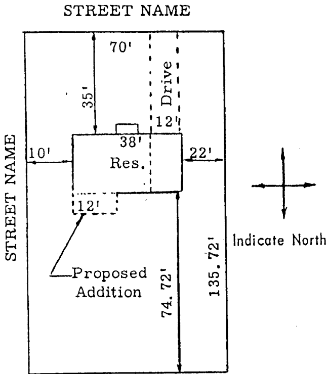
TYPICAL SKETCH
