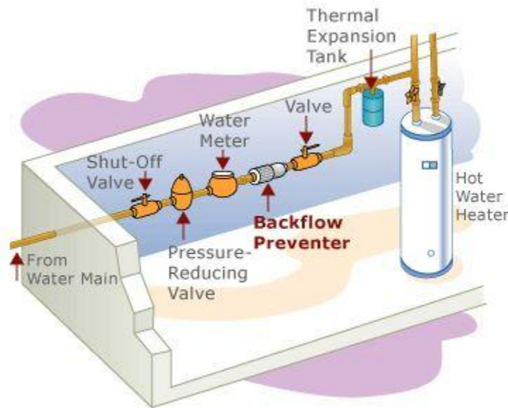
Figure 8 – Interior plumbing near water meter
