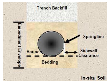
Figure 2 - Embedment Envelope
