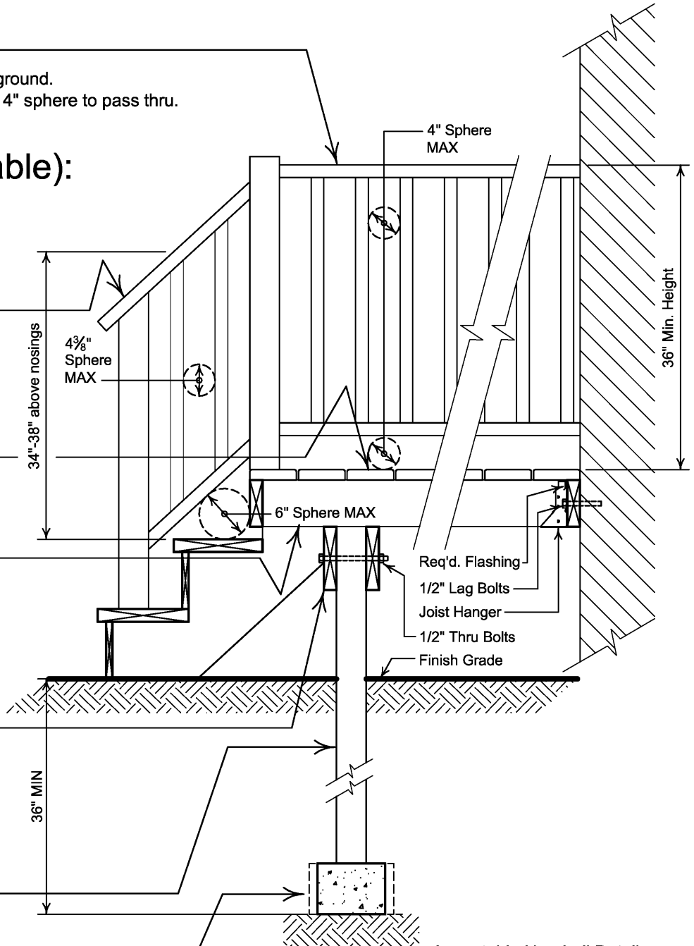
Acceptable Handrail Details:
