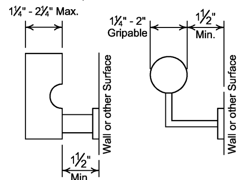
Acceptable Handrail Details:
