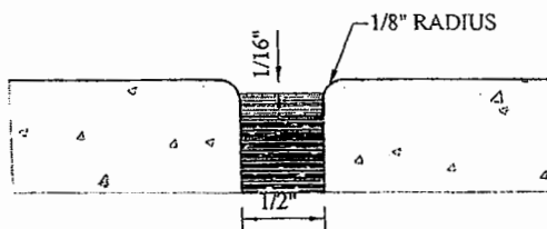
DETAIL EXPANSION JOINT
