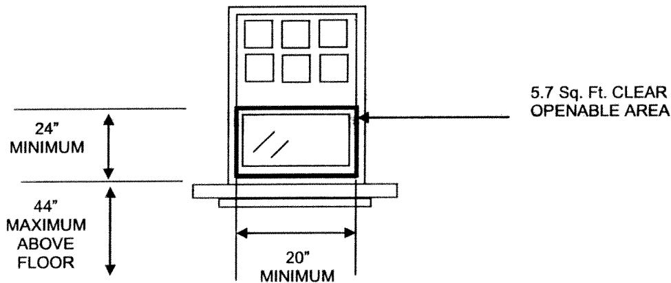
Example of Clear Opening Dimensions
