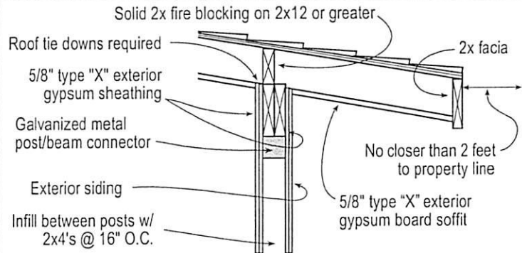
Alternate Detail C - 1 Hour Wall
