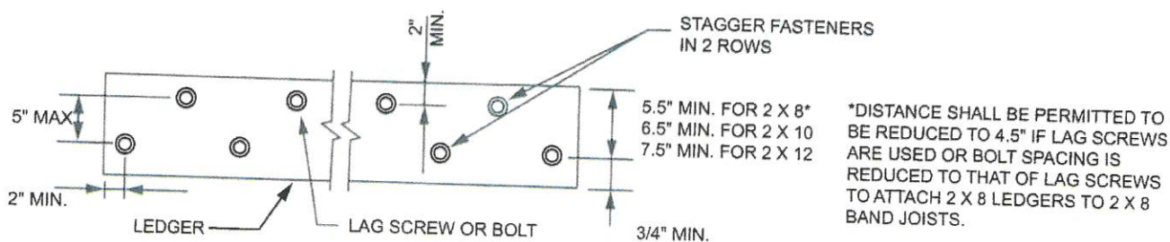
FIGURE 507.9.1.3(1) PLACEMENT OF LAG SCREWS AND BOLTS IN LEDGERS
