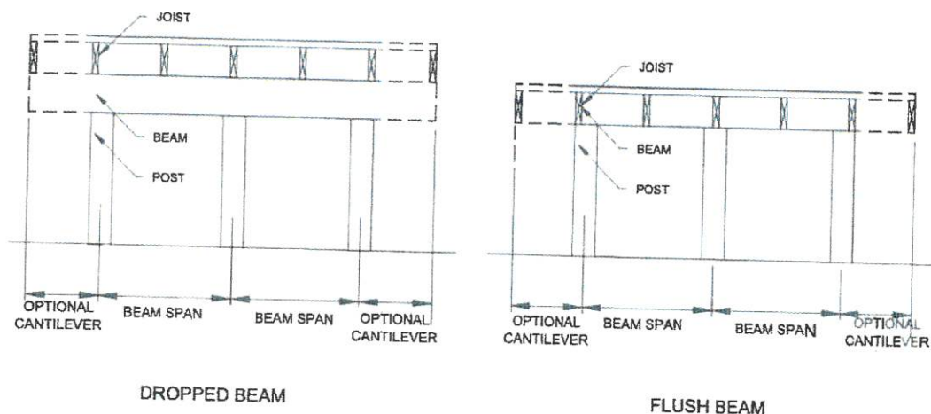
FIGURE 507.5 TYPICAL DECK JOIST SPANS
