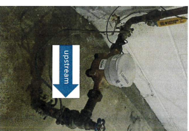
Water meter and service line originating from the floor.
