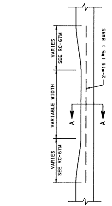
ELEVATION VIEW
