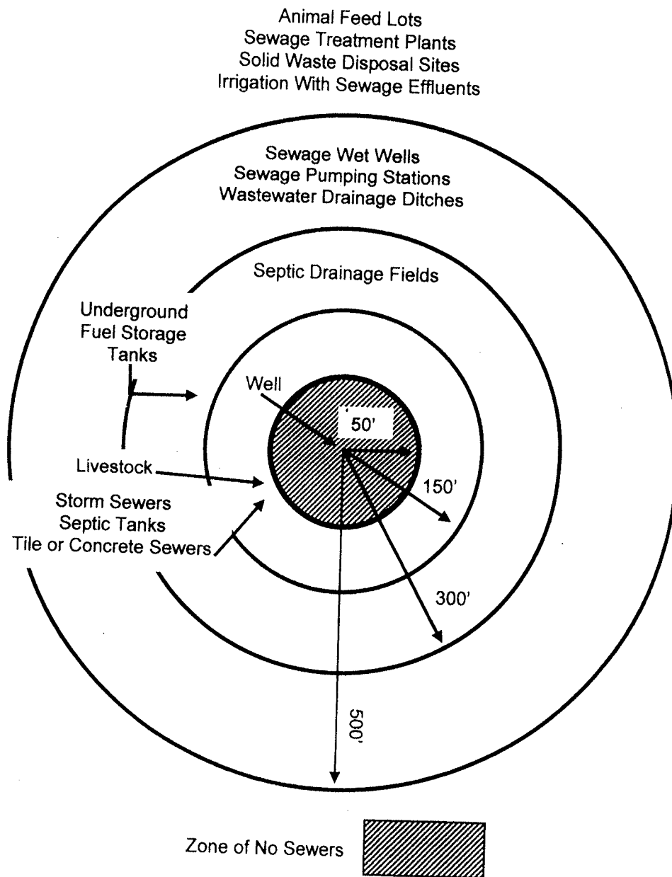
Fig. 4-5 Required Safe Distance from a Well
