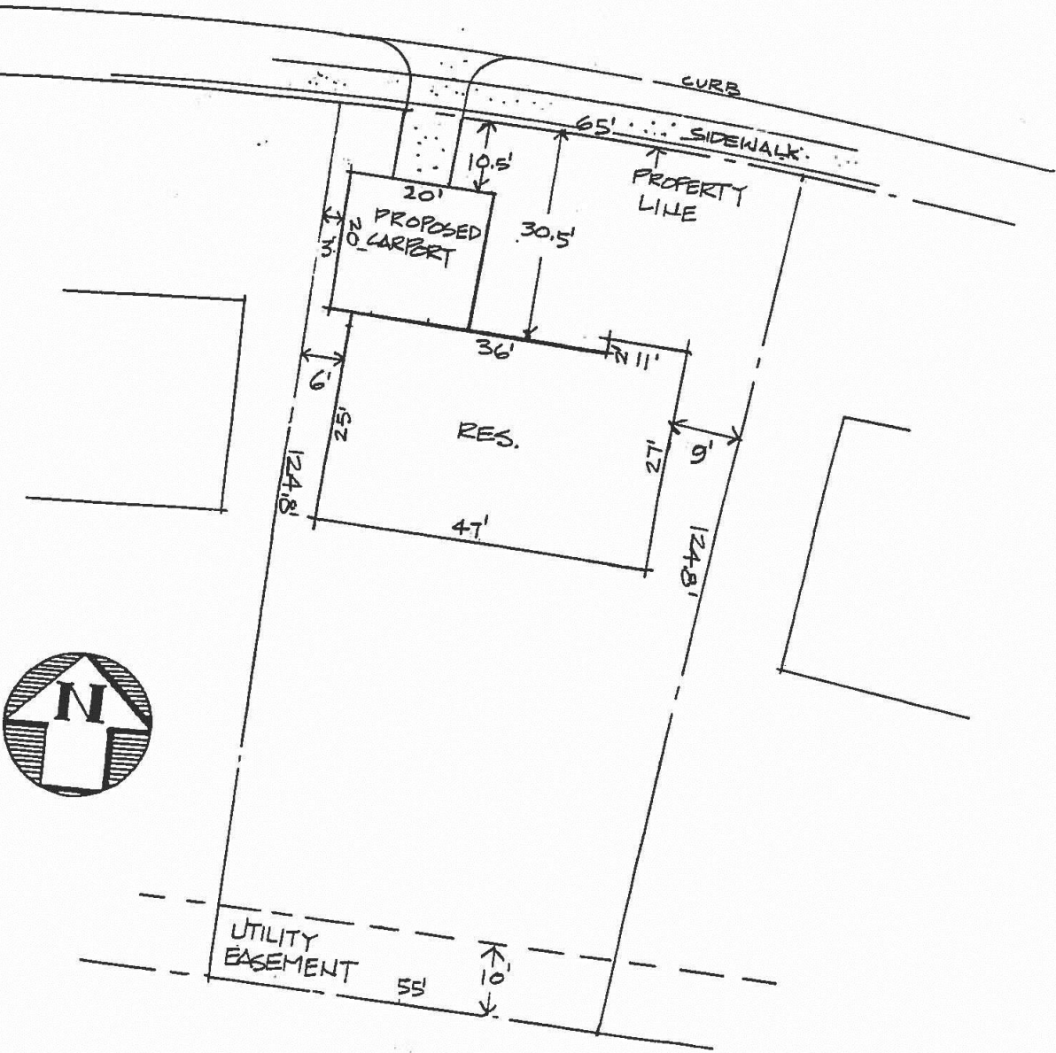
EXAMPLE OF SITE PLAN
