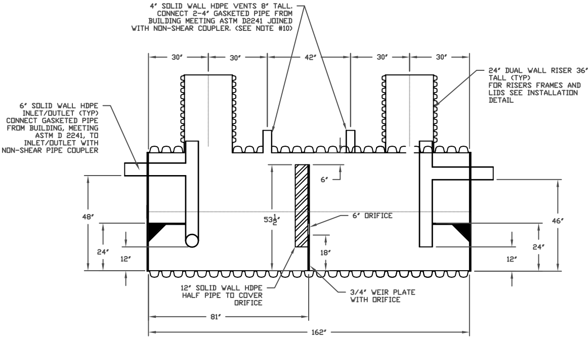
60" DIAMETER - 1500 GALLON GREASE INTERCEPTOR
