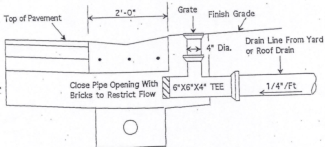
TYPICAL CURB BUBBLER CONCRETE GUTTER CBCG-1
