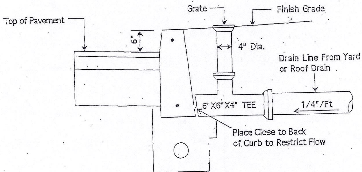
TYPICAL CURB BUBBLER UPRIGHT CURB CBUC-1
